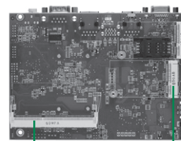
▲ Rear view DDR3L SO-DIMM Full-size PCIe Mini Card
