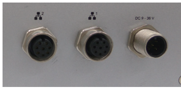
Optional M12 type for DC-in jack and LAN jack
